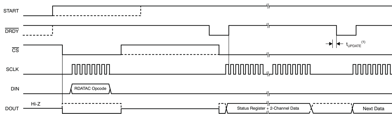
Figure 43. RDATAC Usage
